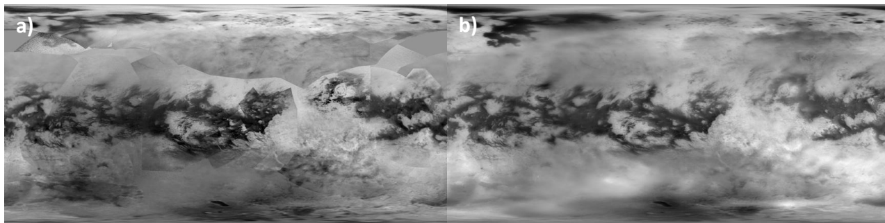
Figure 1: a) Previous Titan mosaic (Cassini image PIA 19658), based on images taken by the Cassini spacecraft's Imaging Science Subsystem (ISS). b) Global mosaic of Titan based on \approx 10000 Cassini ISS images taken in the CB3 filter (938 nm). Image seams were eliminated. Apparent spatial resolution was improved by combining many images, reaching \approx 1 km.
